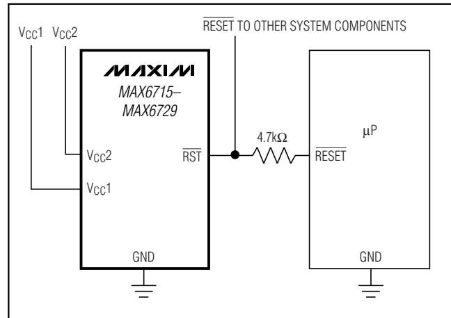
Figure 4. Interfacing to \mu\text{Ps} with Bidirectional Reset I/O
